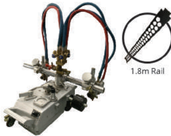
Heavy Duty Gas Cutting Machine TK-12 MAX 2 Cutting Thickness : 6 - 100mm
