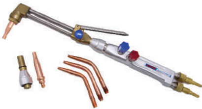
American Type 3 Welding & Cutting Torch
