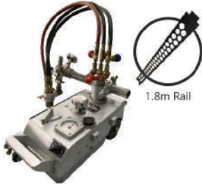
Heavy Duty Gas Cutting Machine TK-12 MAX 1 Cutting Thickness : 6 - 100mm
